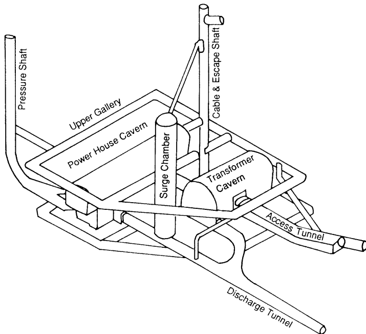
Figure 2. Schematic Presentation of the Project.
