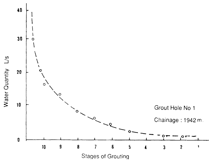
Figure 10. Typical Grouting Effect in Water Quantity Decrease.
