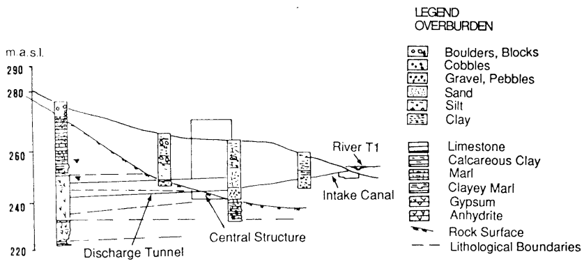
Figure 3. General Geology of the Area at the Lower Intake.
