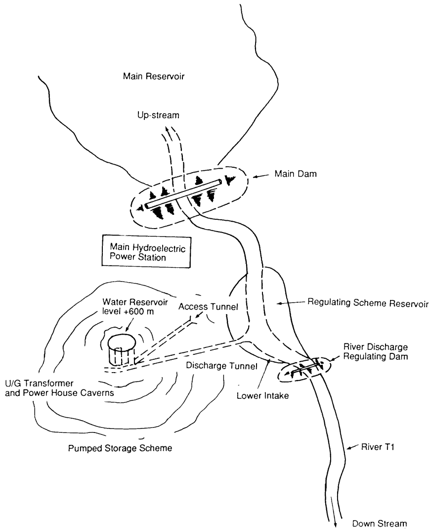
Figure 1. General Layout of the River Development and Pumped Storage Scheme.
