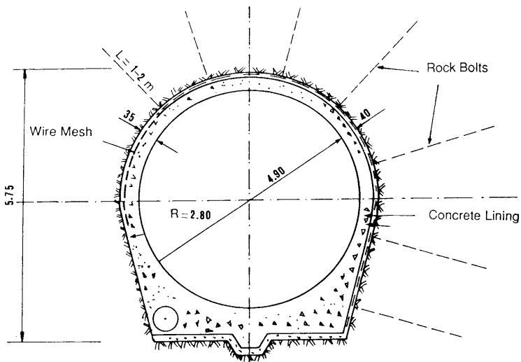
Figure 4. Designed, Finished Profile of Tailrace Tunnel.
