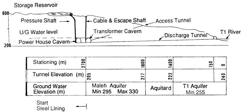
Figure 5. Longitudinal Section of the Pumped Storage Scheme.
